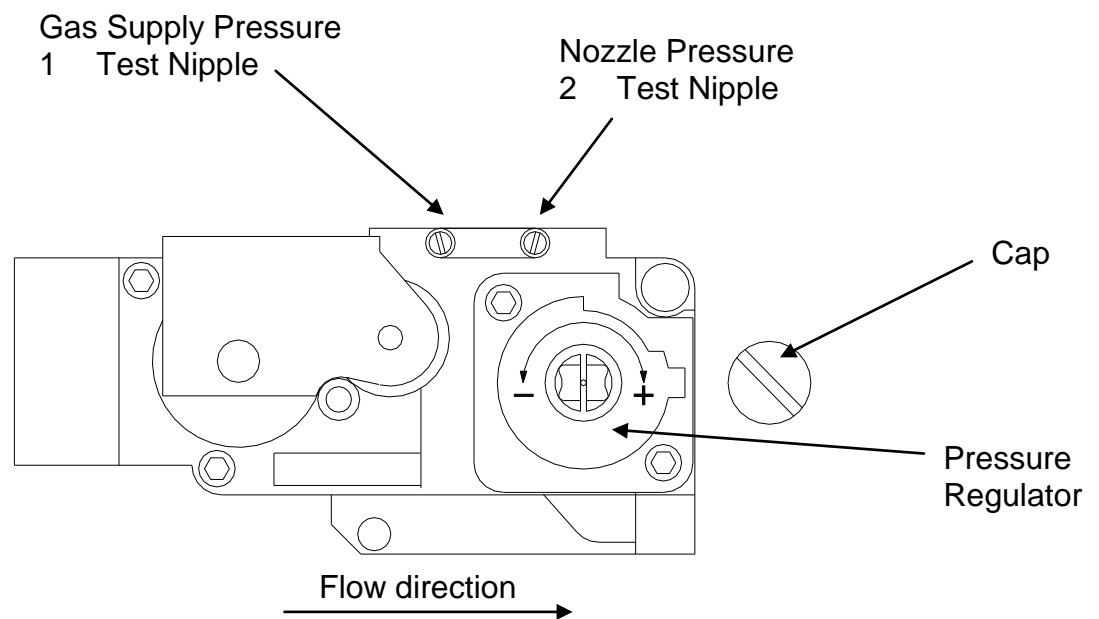
Fig. Combination Valve - Top View
