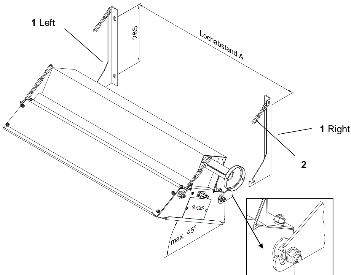
Fig. Heater Mounting
