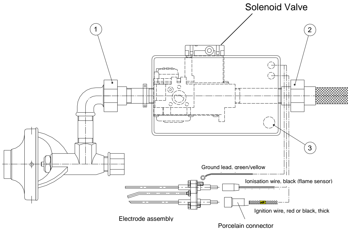
Fig 1. SR 3010-1 (One Stage Layout)
